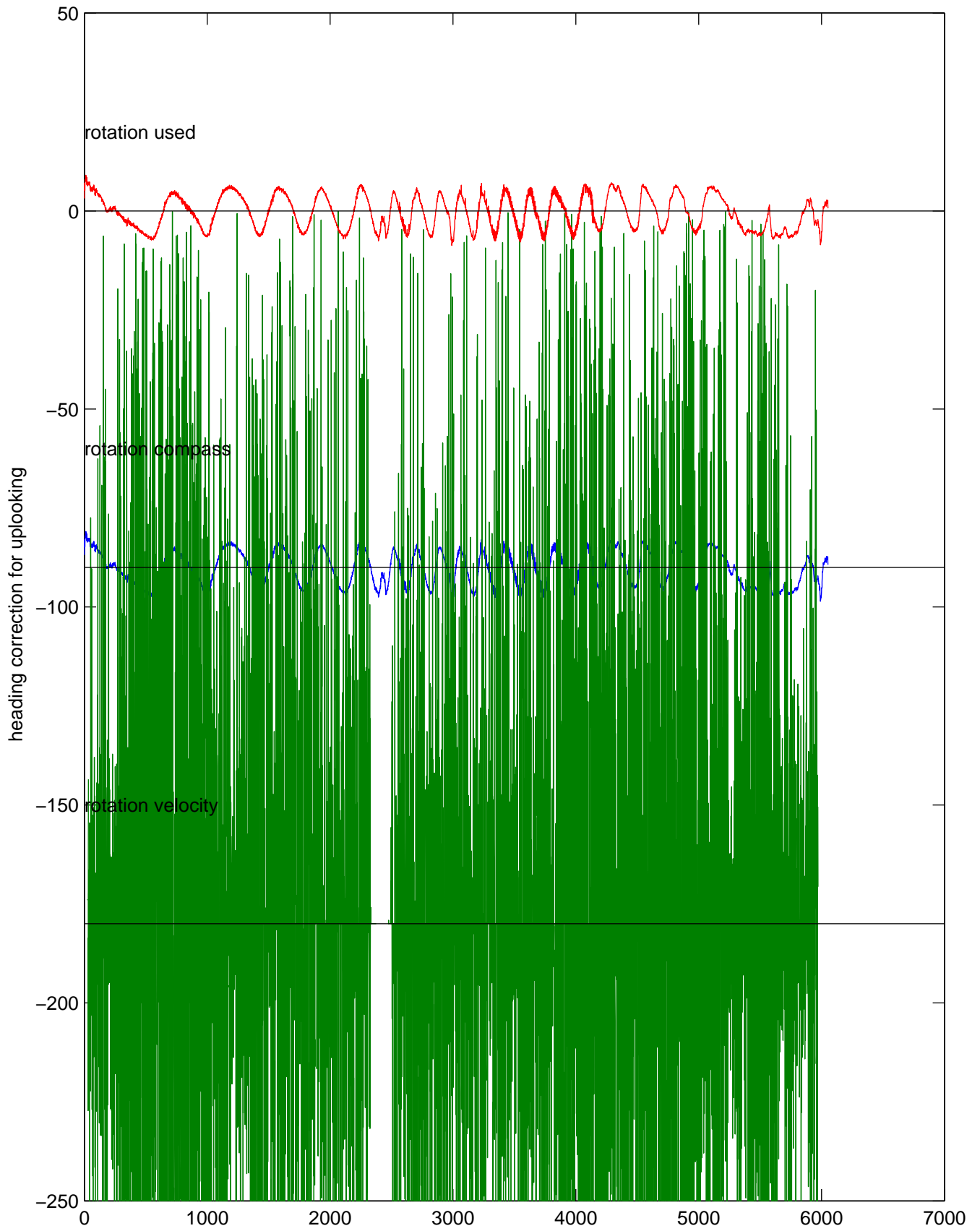
rh11591 (LADCP #171; V5) Figure 5
