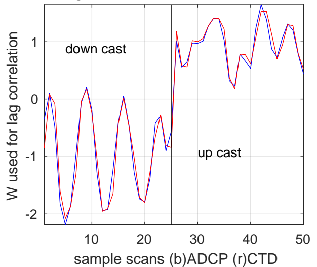
best lag W: 19 scans ~ -19 sec. c:0.98854
