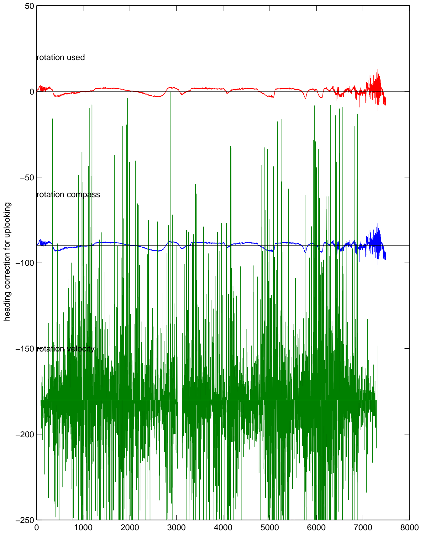
P16N station #56 (V7) Figure 5
