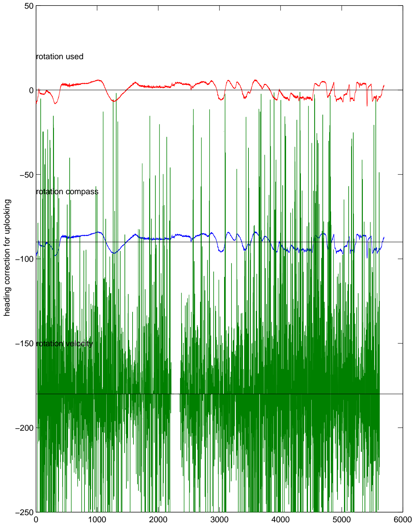
rh11251 (LADCP #135; V5) Figure 5
