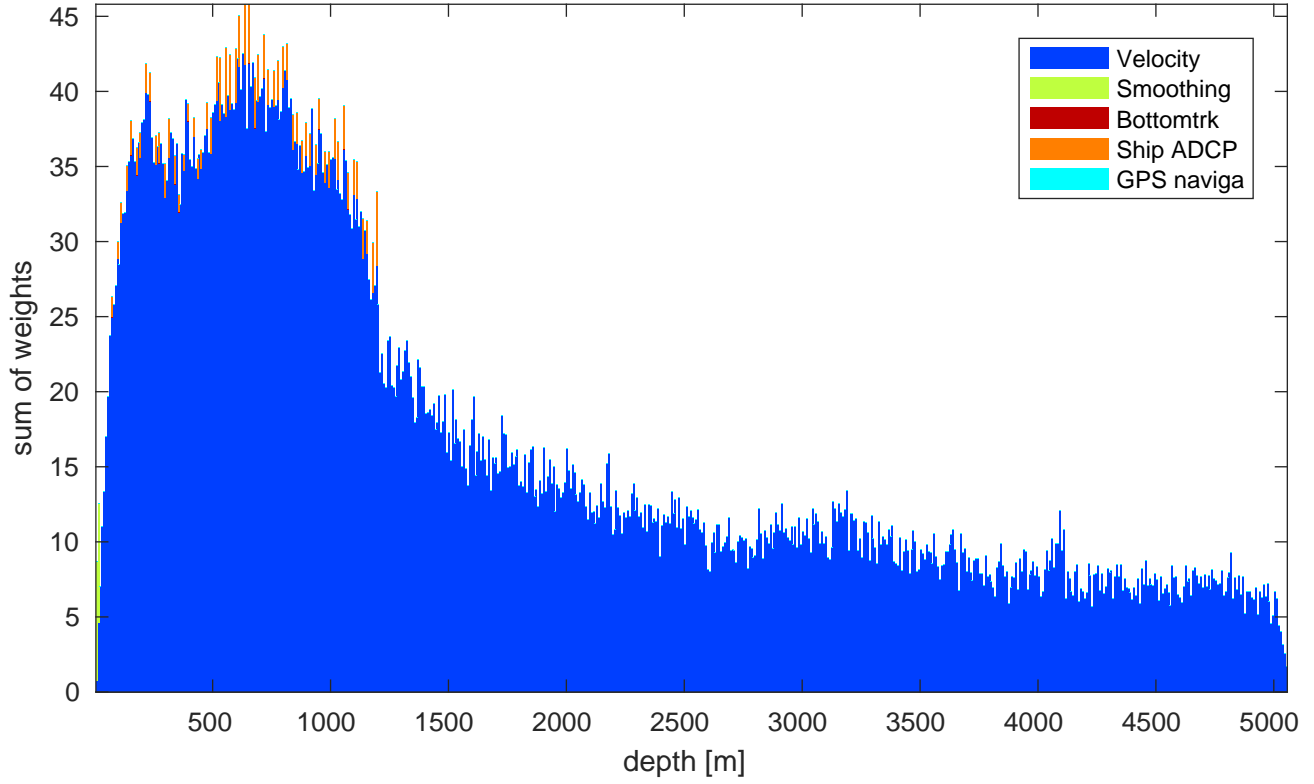
ocean velocity constraints
