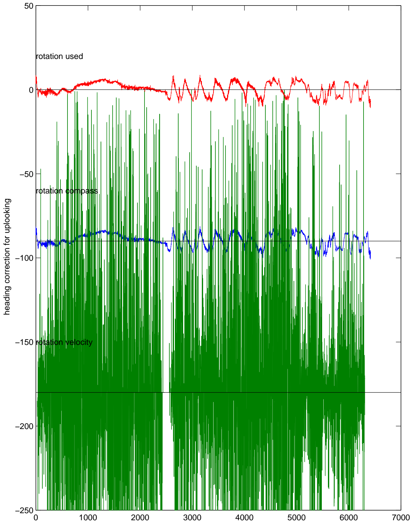
rh11491 (LADCP #161; V5) Figure 5
