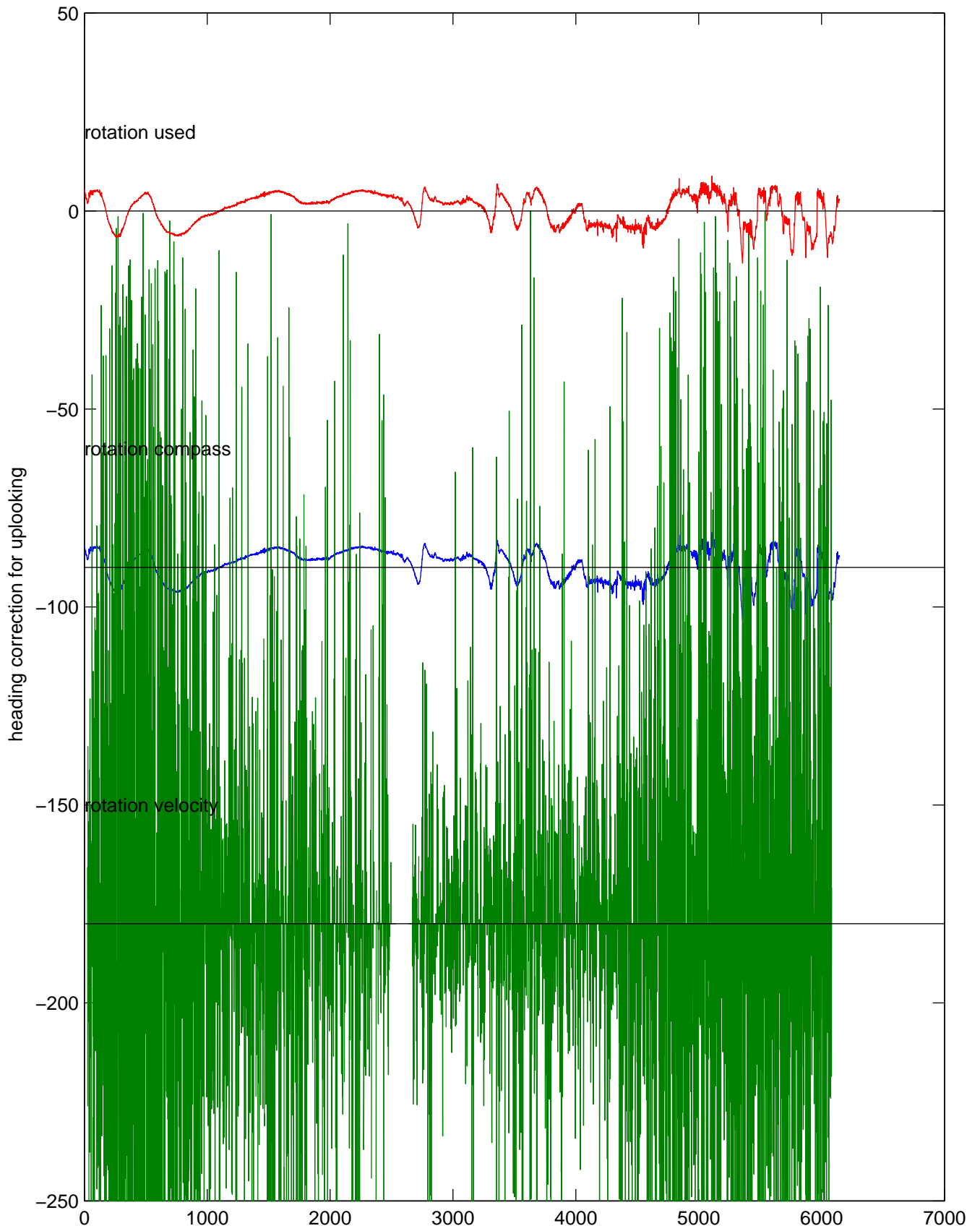
rh11141 (LADCP #122; V5) Figure 5
