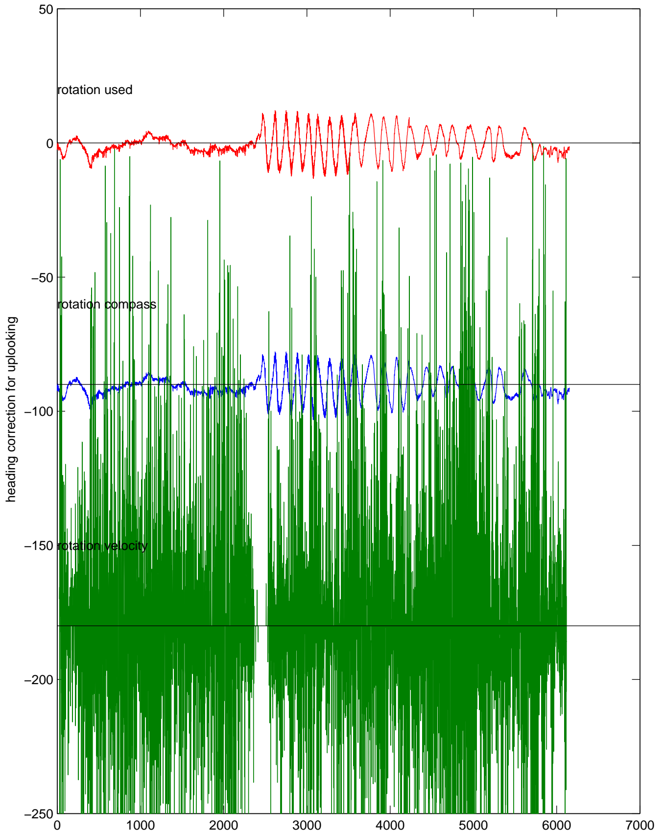
rh11572 (LADCP #169; V5) Figure 5
