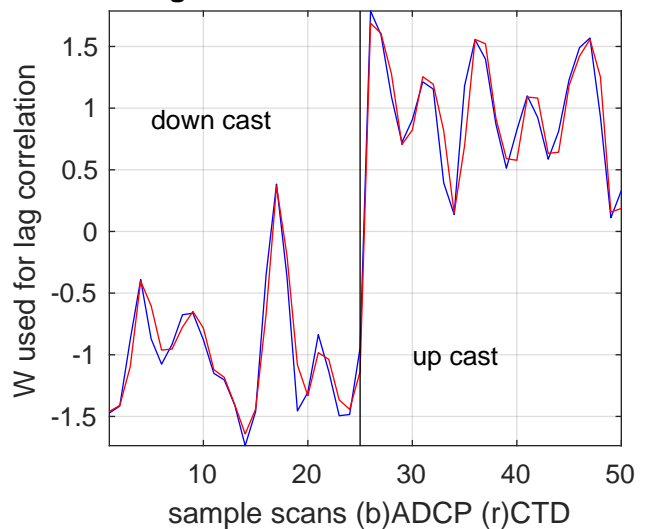
best lag W: 14 scans ~ -14 sec. c:0.99081
