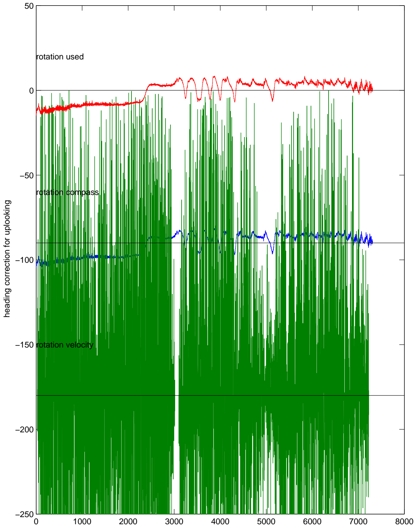
rh12011 (LADCP #214; V5) Figure 5
