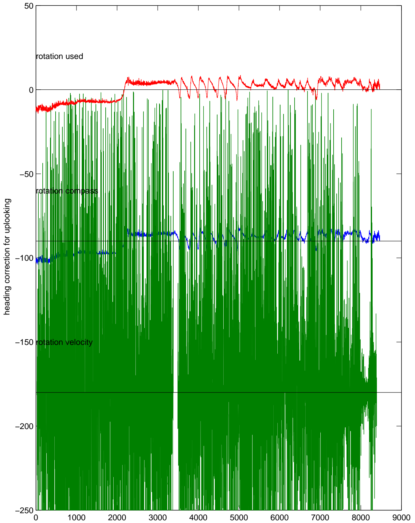
rh11891 (LADCP #202; V5) Figure 5
