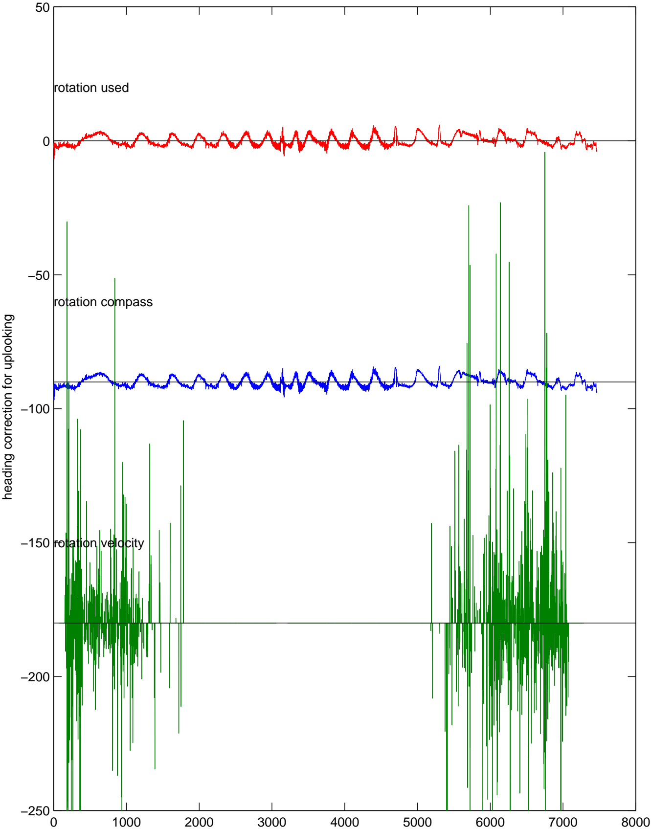
P16N station #144 (V7) Figure 5
