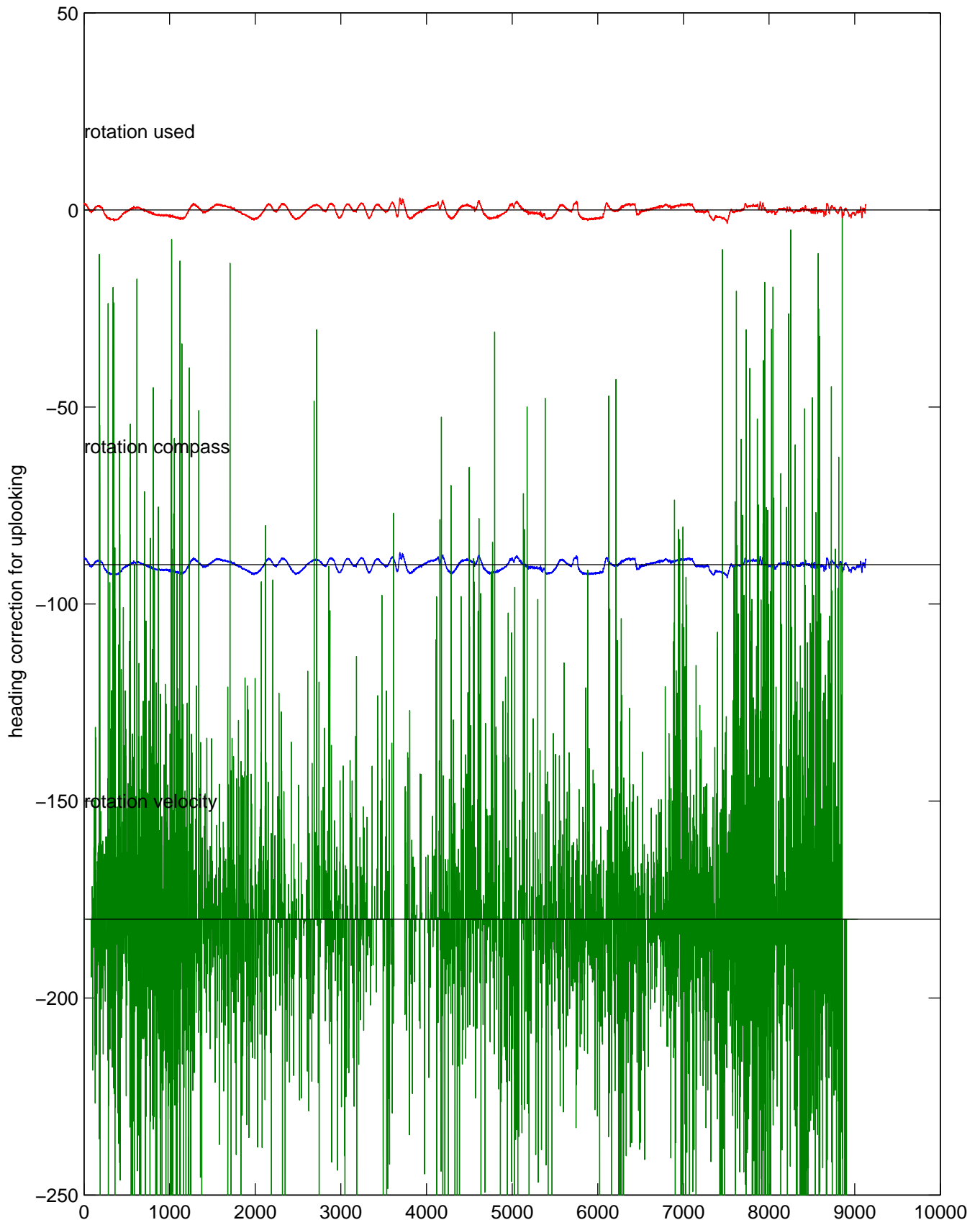
P16N station #22 (V7) Figure 5
