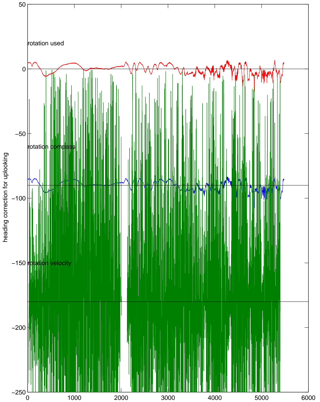
rh10751 (LADCP #083; V5) Figure 5
