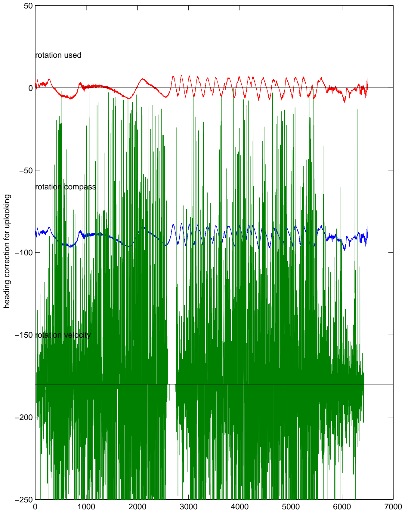
rh11651 (LADCP #178; V5) Figure 5
