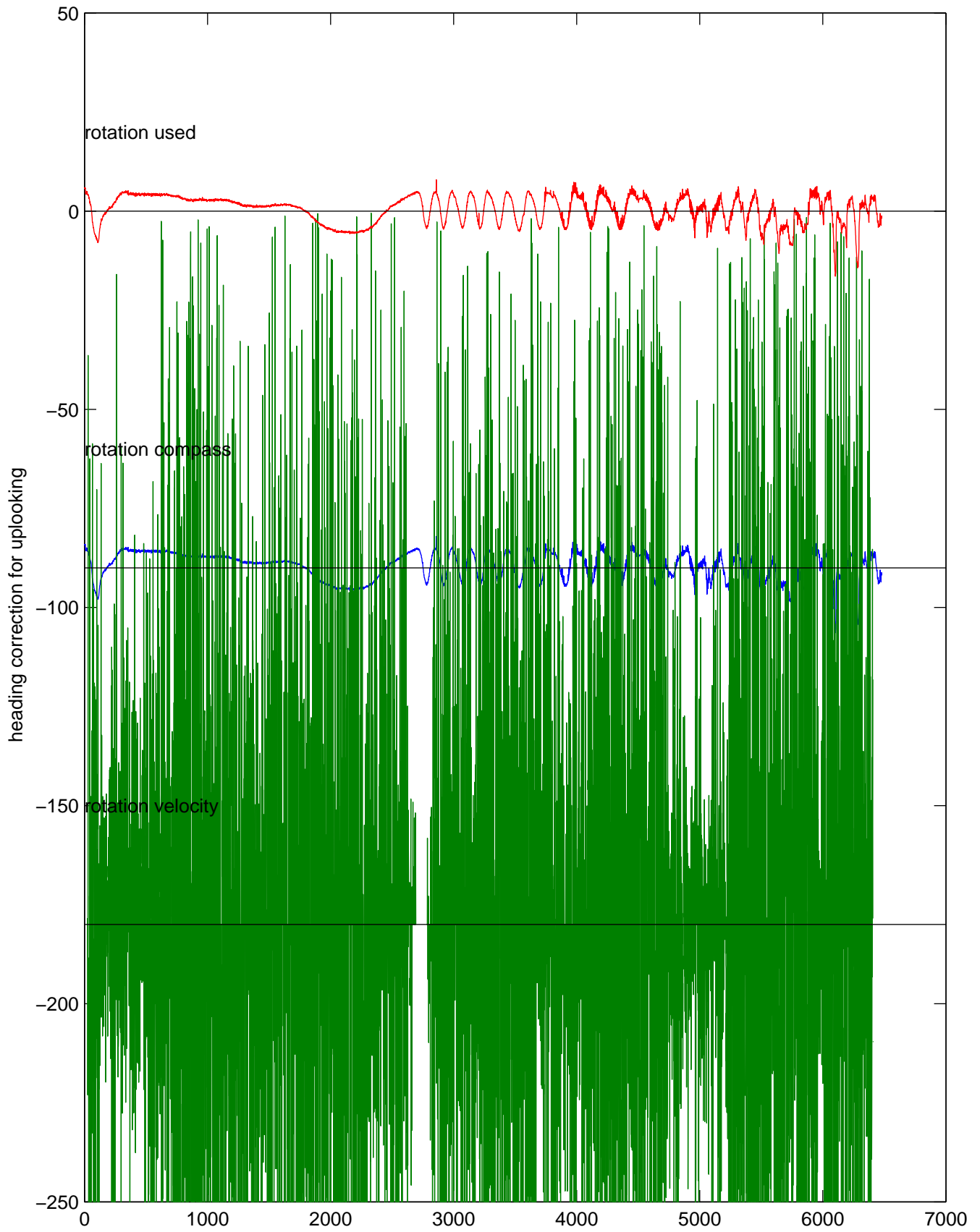
rh10901 (LADCP #098; V5) Figure 5
