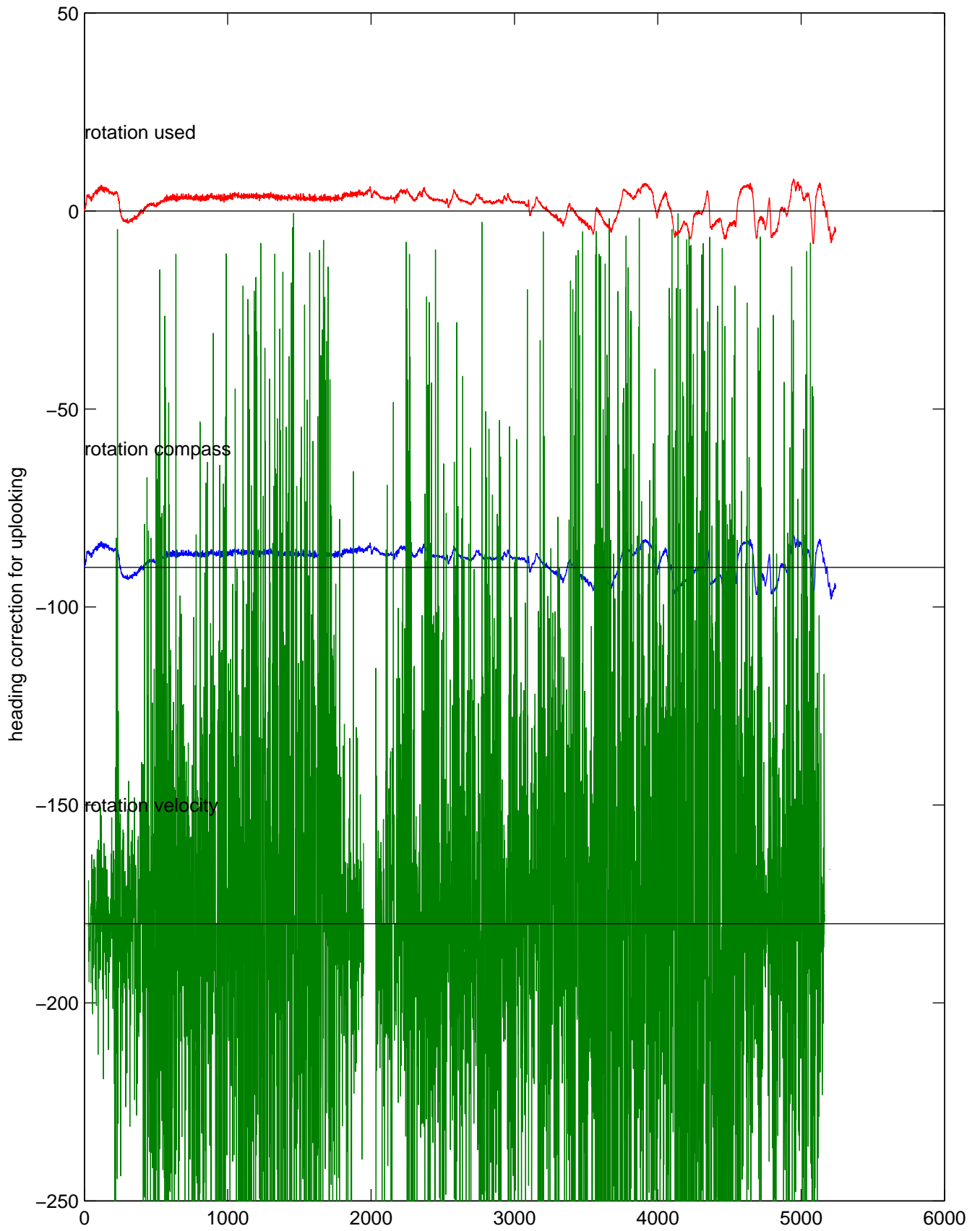
rh11391 (LADCP #151; V5) Figure 5
