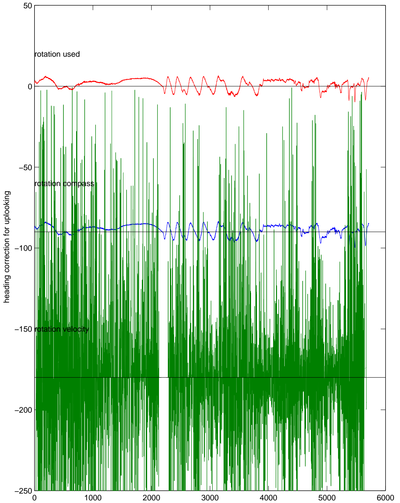
rh11211 (LADCP #131; V5) Figure 5
