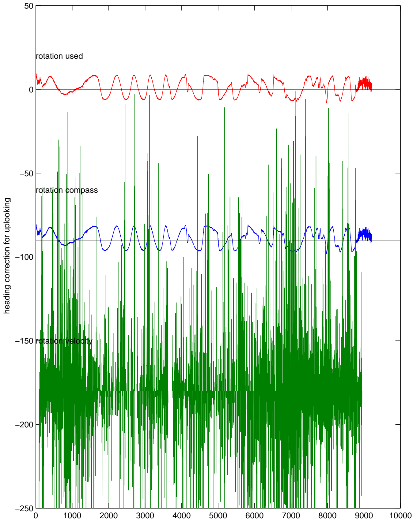
P16N station #76 (V7) Figure 5
