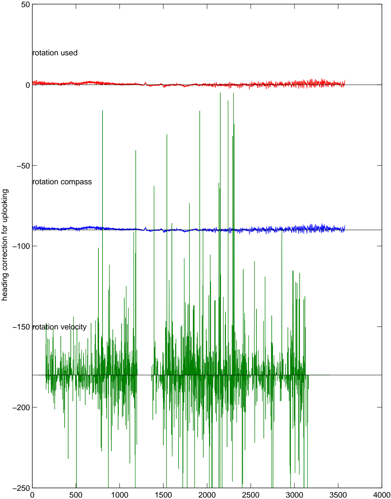
P16N station #185 (V7) Figure 5
